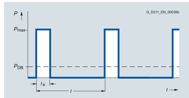
Load diagram for the braking resistors
