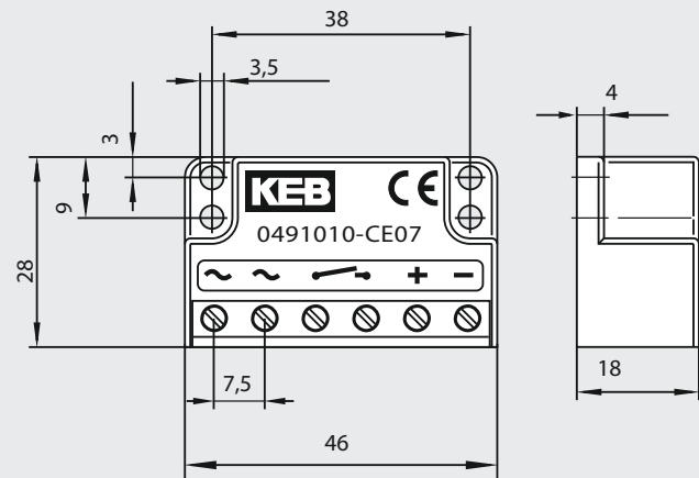
Terminal cross section 2,5 mm 2
