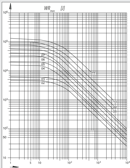
Friction switching frequency Type M, T
