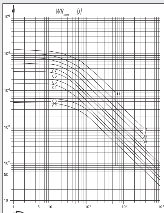
Friction switching frequency Type M, T
